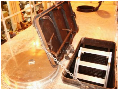
Marine Hatch and Ship's Ladder
